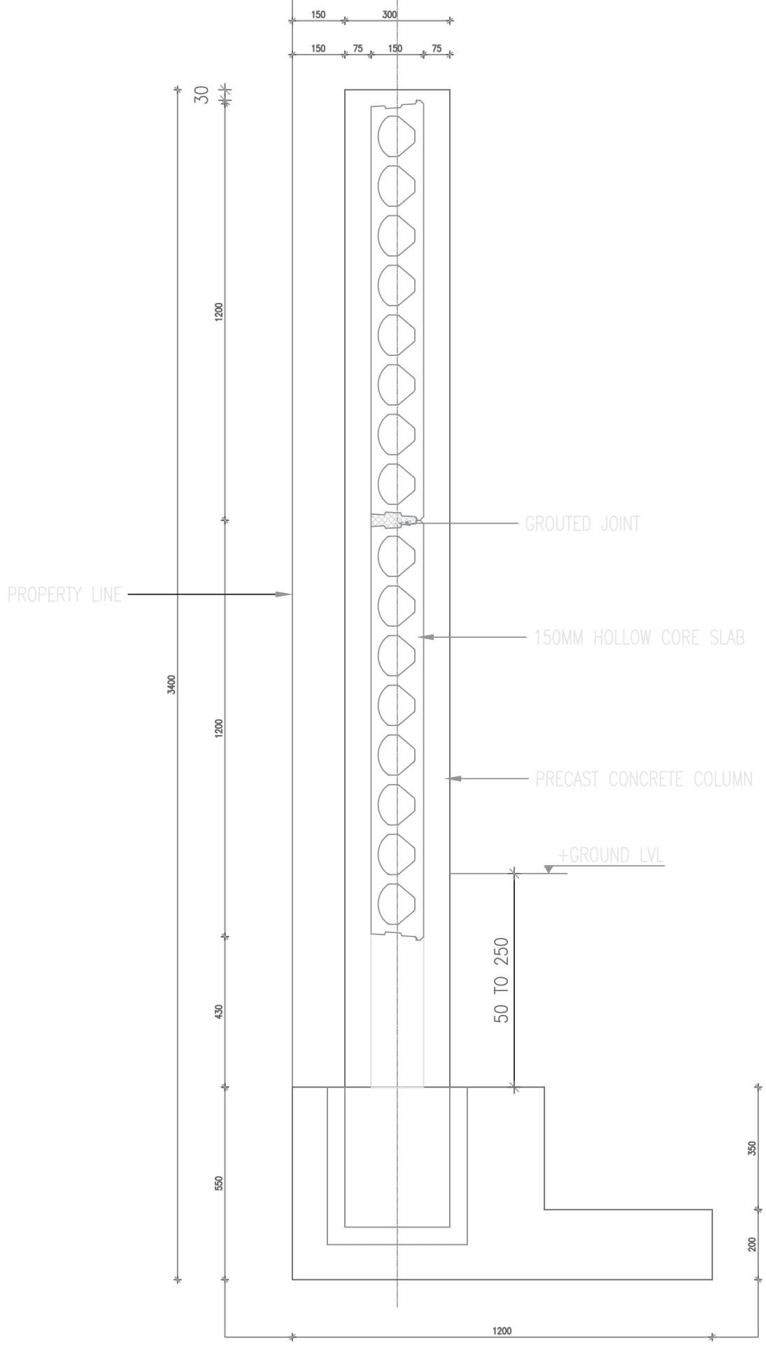
BOUNDARY WALL TYPE-3
